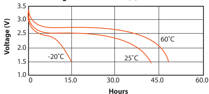
Discharge Characteristics (II) Current: 800mA-cont
