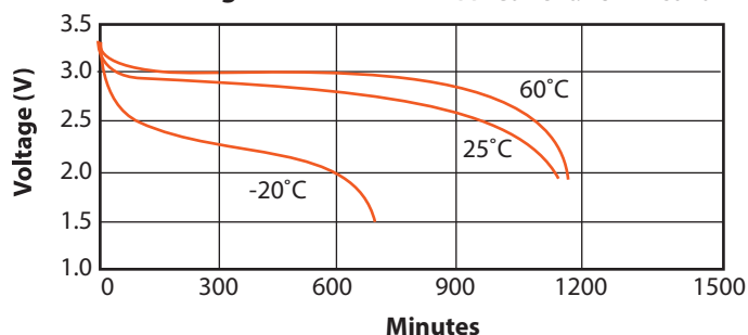
Discharge Characteristics (I) Current: 45mA-cont
